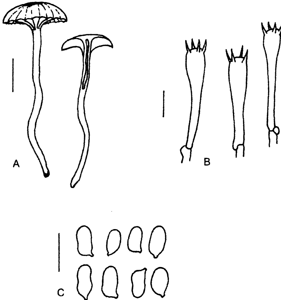
Figure 2. Hygrocybe julietae (hb. Young 2014; BRI). A habit; B basidia; C spores. Habit and T/S sketch, bar = 10 mm; microcharacters, bar = 10 µm.
