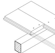
2 nails a joist over 85mm cover
