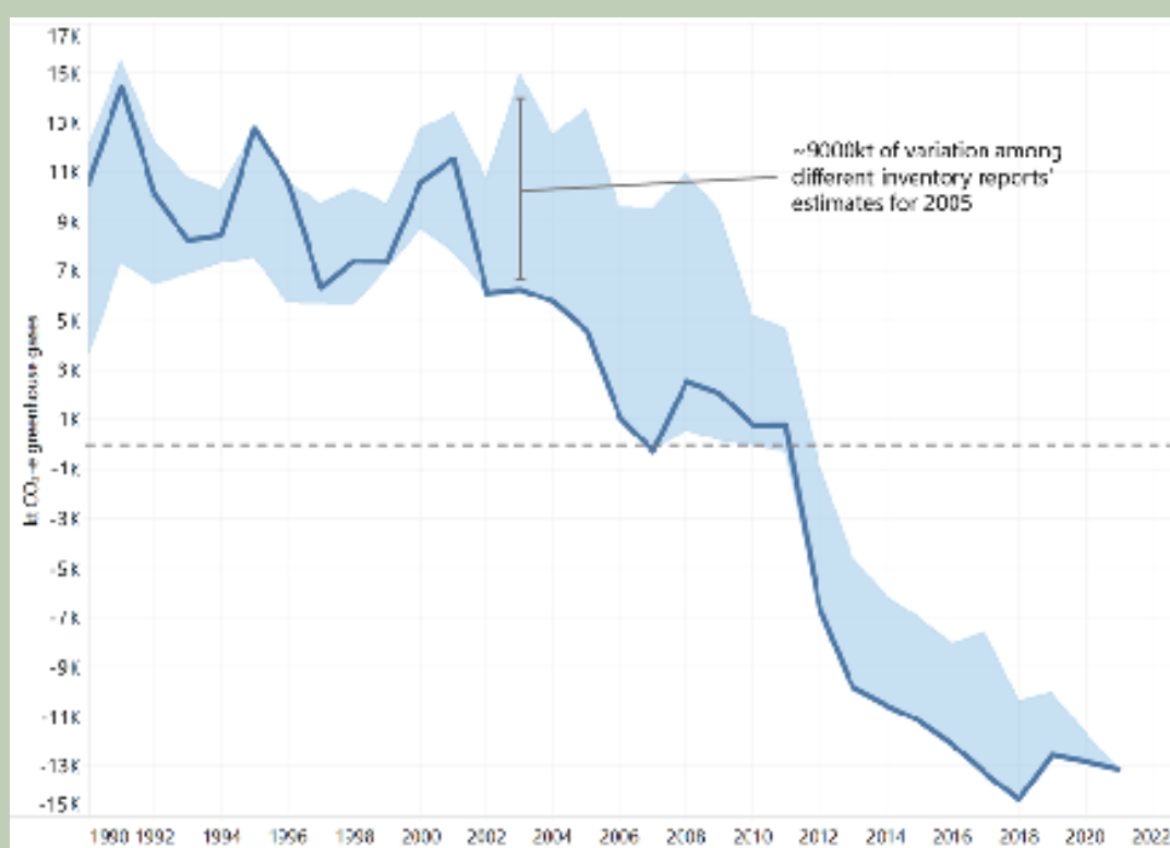
Figure 5: Comparing Tasmania's LULUCF Emissions as reported in STGGIs since 2008
